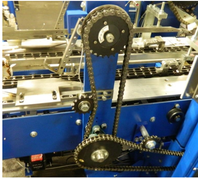
Vertical flap tucker design for dependable tray sealing
